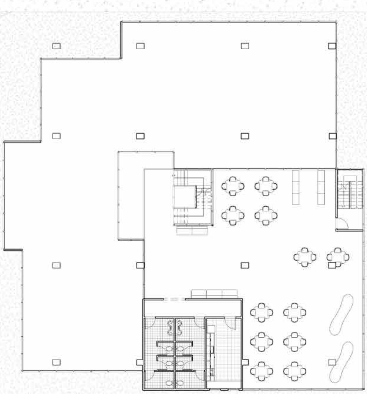
Level 2 1/16" = 1'-0"
