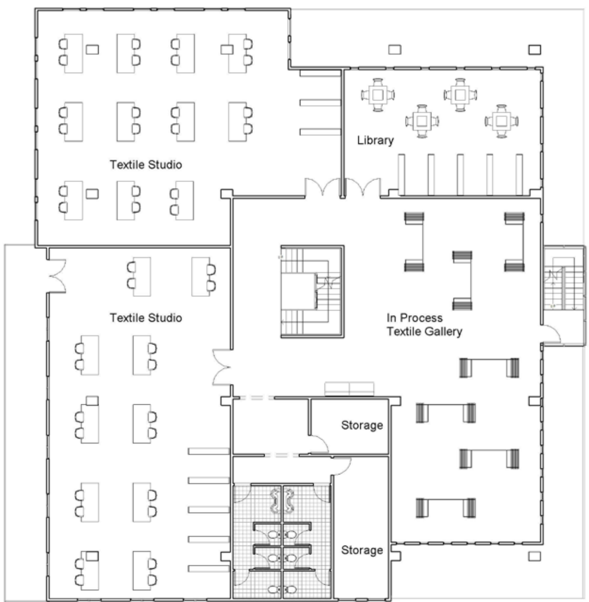
Level 4 1/16" = 1'-0"
