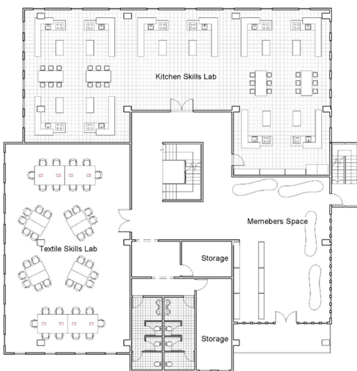
Level 7 1/16" = 1'-0"
